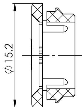
SECTION Y-Y
