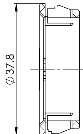
SECTION Y-Y
