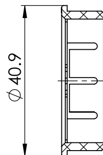
SECTION Y-Y
