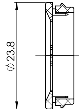
SECTION Y-Y
