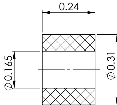
SECTION Y-Y
