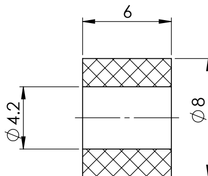
SECTION Y-Y
