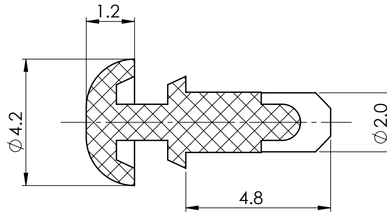
SECTION Y-Y
