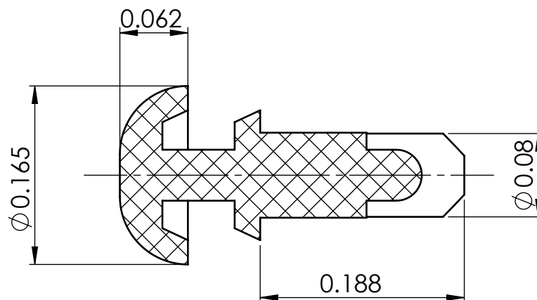
SECTION Y-Y
