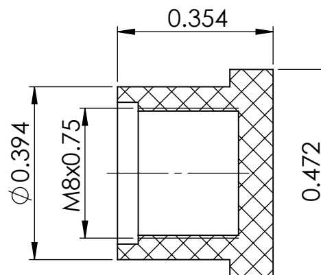
SECTION Y-Y
