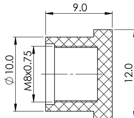
SECTION Y-Y
