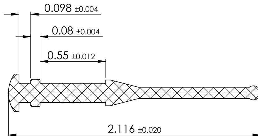
SECTION X-X
