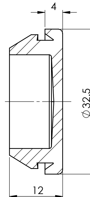
SECTION Y-Y
