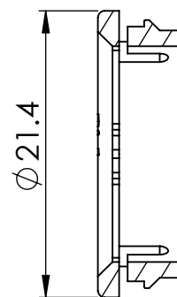
SECTION Y-Y
