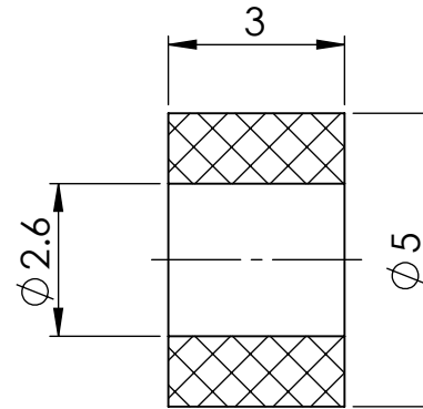
SECTION Y-Y
