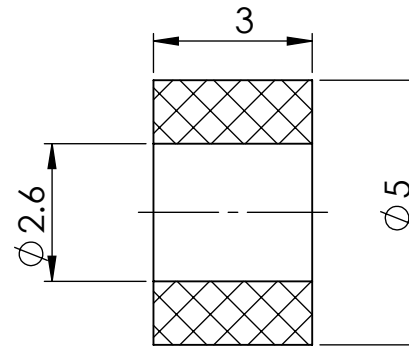
SECTION Y-Y
