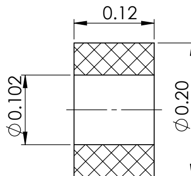
SECTION Y-Y
