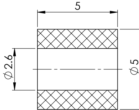
SECTION Y-Y
