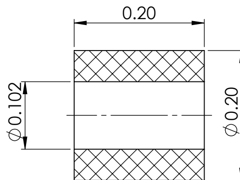
SECTION Y-Y
