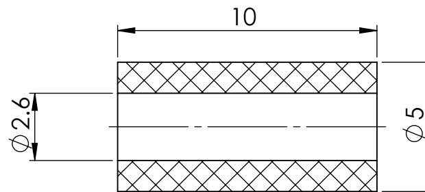
SECTION Y-Y
