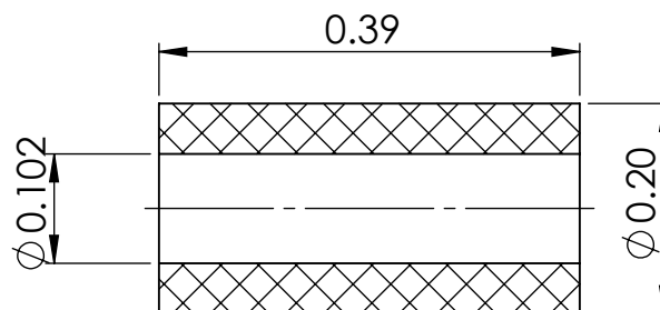
SECTION Y-Y
