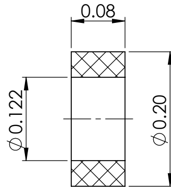
SECTION Y-Y
