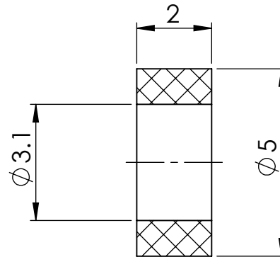
SECTION Y-Y
