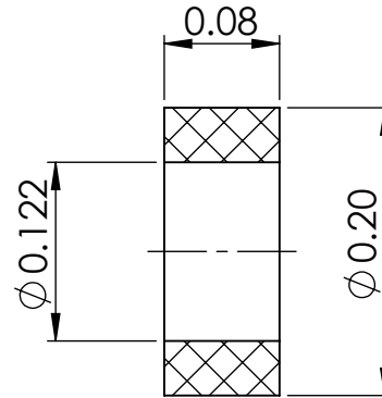
SECTION Y-Y
