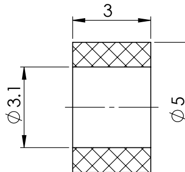
SECTION Y-Y
