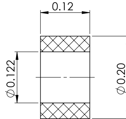
SECTION Y-Y
