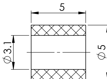
SECTION Y-Y
