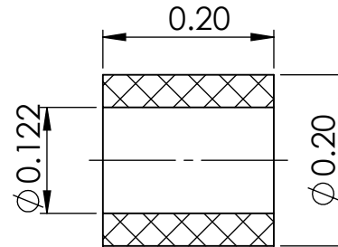
SECTION Y-Y
