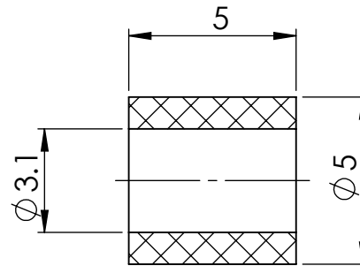
SECTION Y-Y
