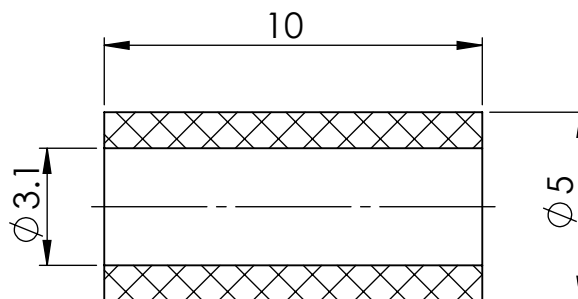
SECTION Y-Y
