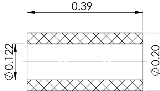
SECTION Y-Y
