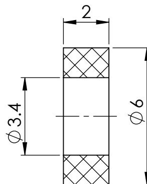
SECTION Y-Y
