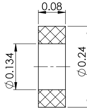
SECTION Y-Y
