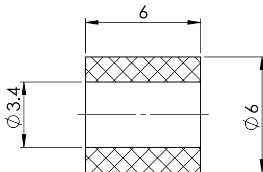
SECTION Y-Y
