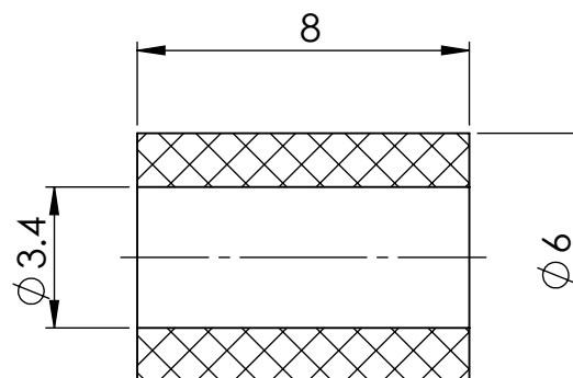
SECTION Y-Y
