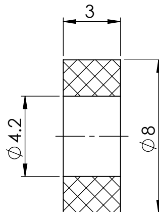
SECTION Y-Y
