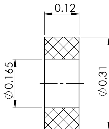
SECTION Y-Y
