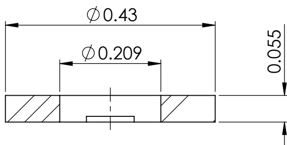
SECTION X-X
