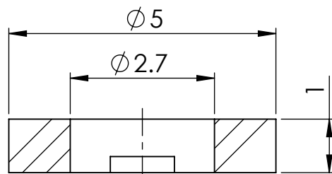
SECTION X-X
