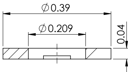
SECTION X-X
