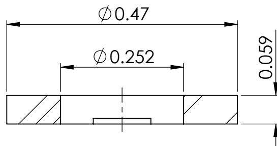
SECTION X-X
